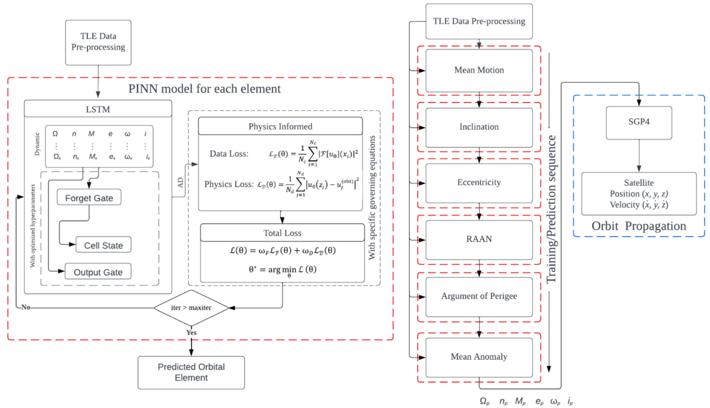
Fig. 3. Overview of the proposed PINN framework integrating LSTM for orbital parameter prediction. The model sequentially predicts each orbital element using TLE-derived features, incorporating both \mathcal{L}_F and \mathcal{L}_D . The predicted elements are used with SGP4 for satellite state estimation.
