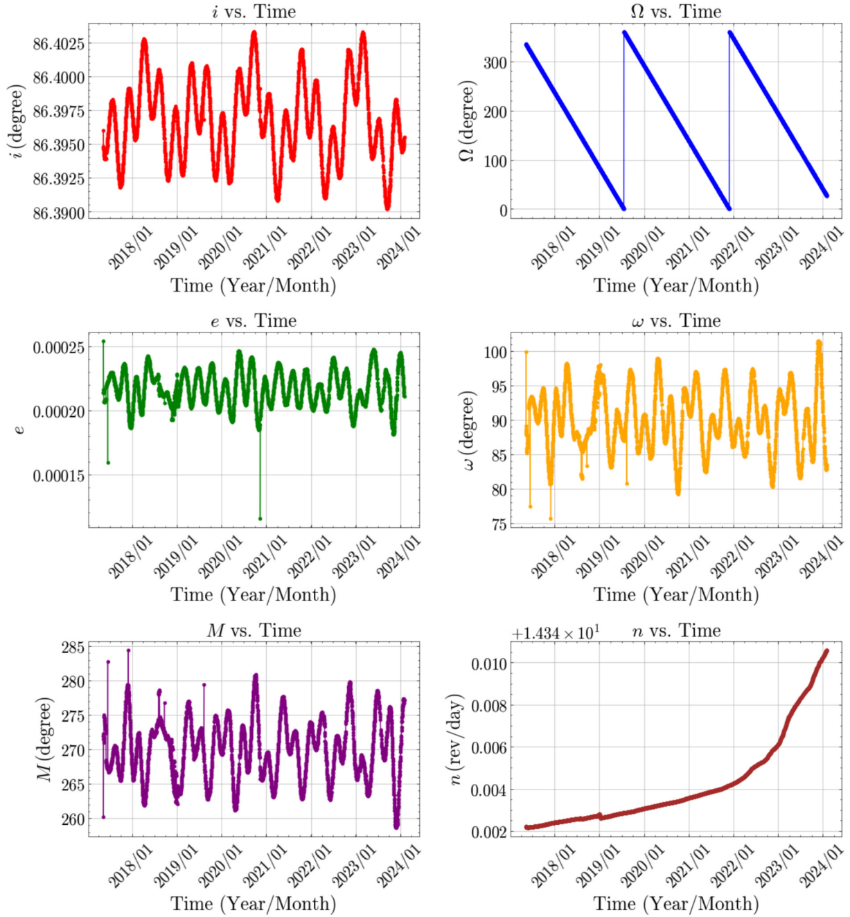
Fig. 4. Temporal evolution of orbital elements from the last 5000 IRIDIUM 7 TLE records.
