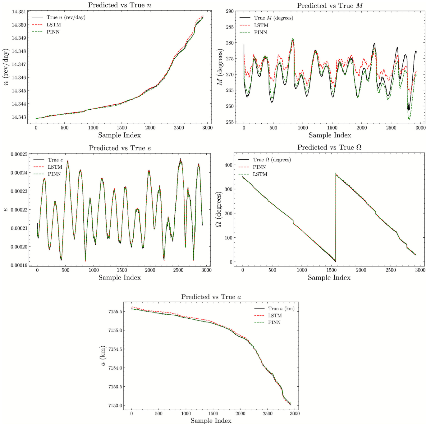
Fig. 7. Comparison of LSTM and PINN predictions against true orbital parameters: n , \Omega , e , M and a for IRIDIUM 7. The plots illustrate the advantage of integrating physics-informed constraints within PINNs, particularly evident in improved long-term accuracy and stability.
