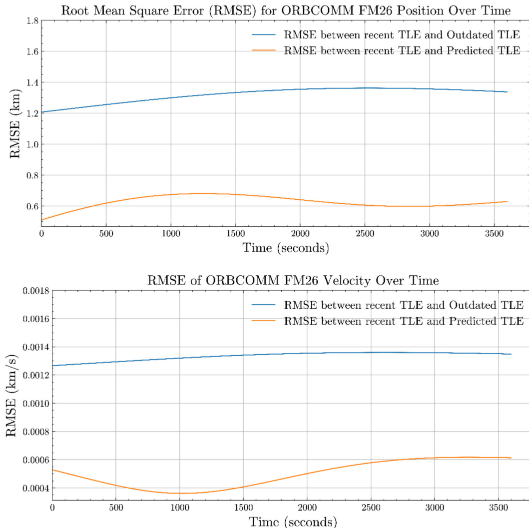
Fig. 11. RMSE for ORBCOMM FM26 position and velocity over time, comparing the recent TLE with predicted TLE and an outdated TLE.
