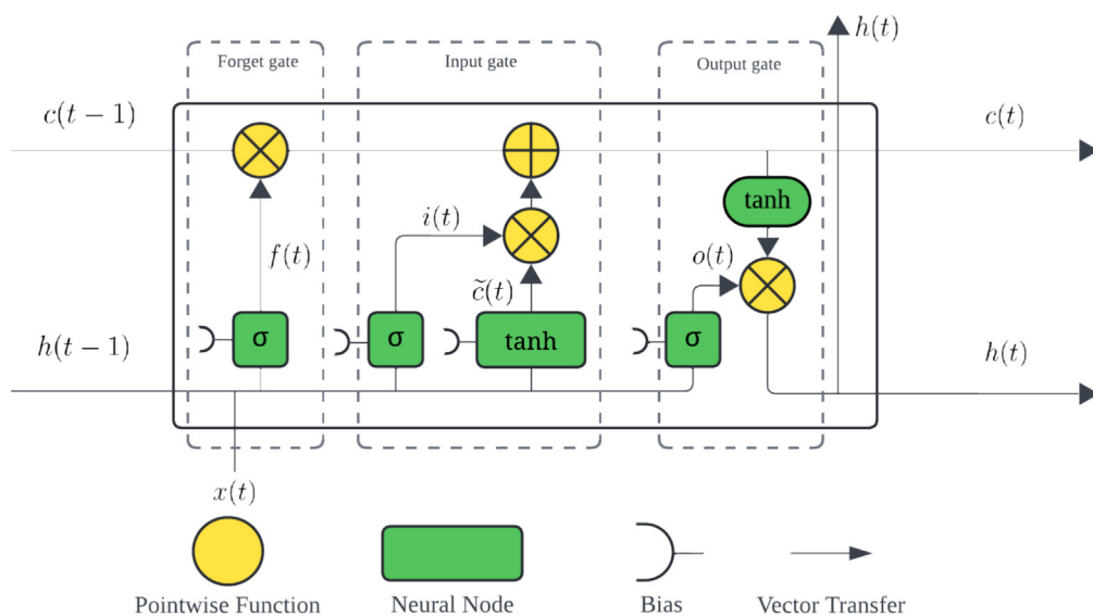
Fig. 1. This figure illustrates an LSTM cell's structure and data flow. The Forget Gate (left) computes f(t) to determine what information to discard from the previous cell state c(t-1) . The Input Gate (middle) decides what new information to add to the cell state by computing it and generating candidate values \tilde{c}(t) , updating the cell state to c(t) . The Output Gate (right) determines the output hidden state by computing o(t) and producing h(t) ( Mahmud et al., 2024 ).
