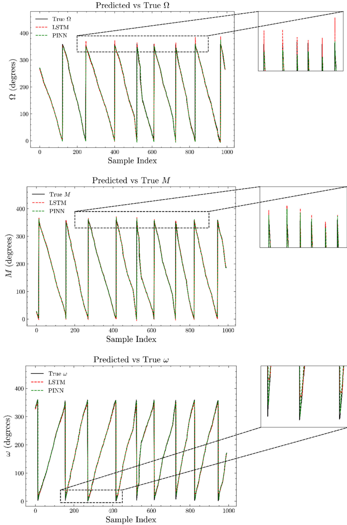
Fig. 10. Predicted vs. true \Omega , M and \omega for ORBCOMM FM26 using LSTM and PINN against the TLE reference. The inset zooms on the 0–360° wrap-around regions, where PINN delivers smoother, more continuous transitions and suppresses the abrupt discontinuities seen in the LSTM outputs.
