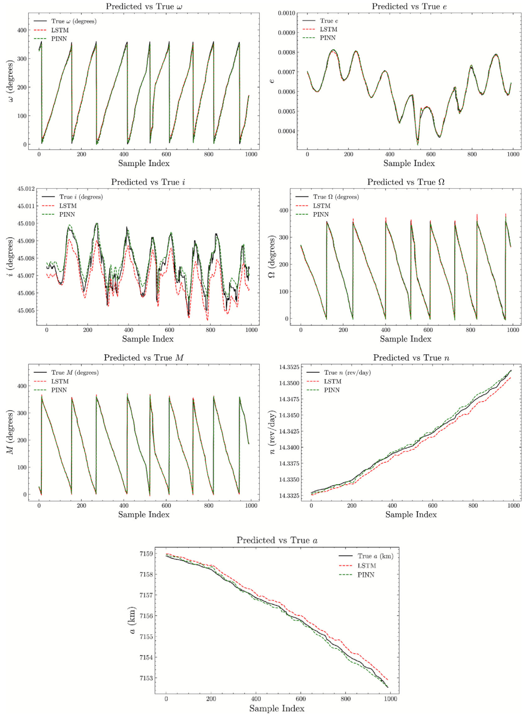
Fig. 9. Comparison showing LSTM predictions and PINN predictions for the orbital elements of ORBCOMM FM26 over 1000 epochs.
