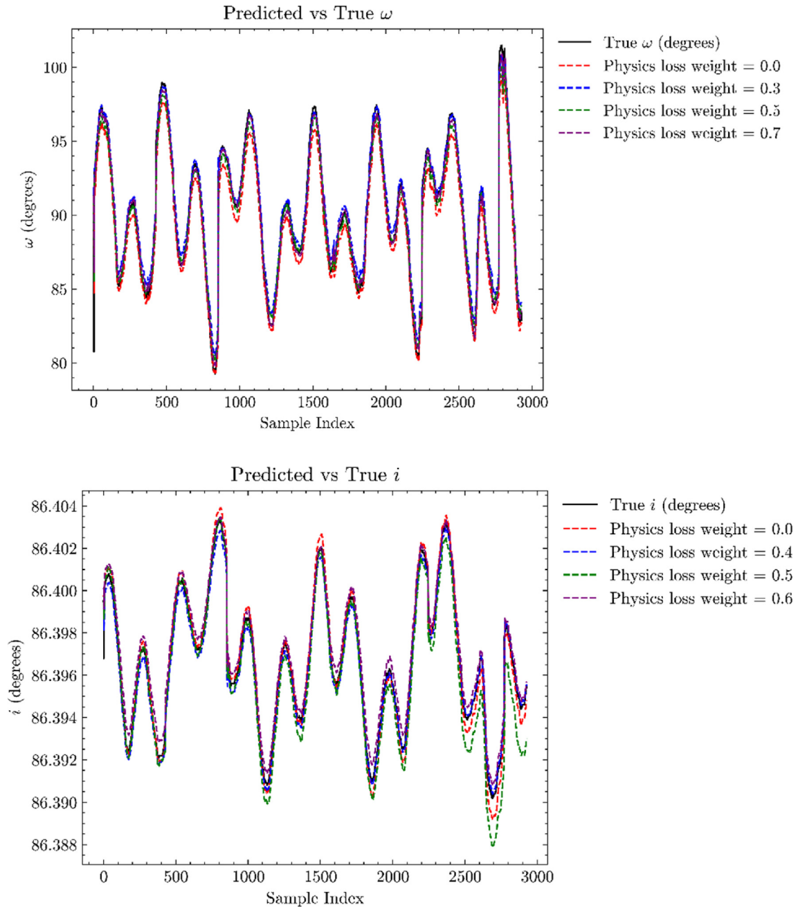
Fig. 6. Time-series comparison of the PINN predictions for \omega and i under different physics loss weight settings for IRIDIUM 7.
