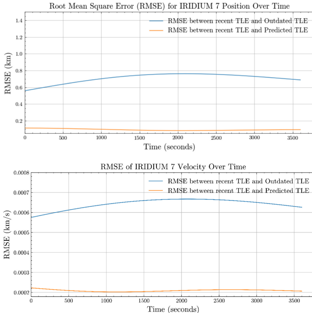
Fig. 8. RMSE for IRIDIUM 7 position and velocity over time, comparing the recent TLE with predicted TLE and an outdated TLE.
